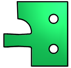
182-160 insert Uses 161 backer #6 Quarter Round Bead profile
