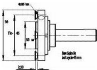
S1 - Saw Blade 30mm x 45mm
